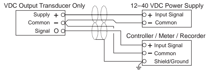
Figure 4 – Wiring for VDC Pressure Transducers when applied with External DC Supply
